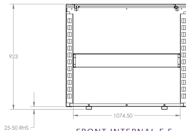
FRONT INTERNAL F-F SECTION VIEW
